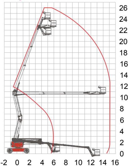
Range of motion HZ260JRT
